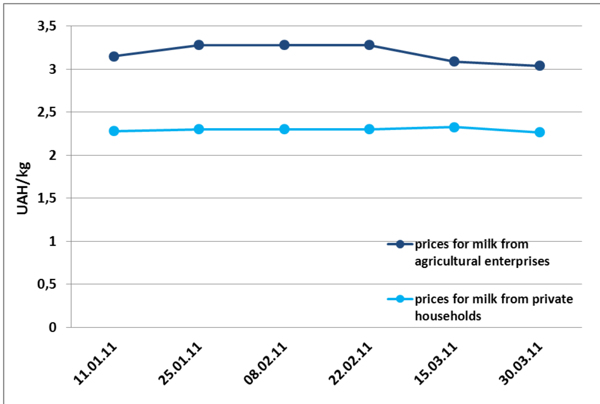
Fig. 2. Dynamics of prices for milk in Ukraine in terms of weeks (processing enterprises data)
