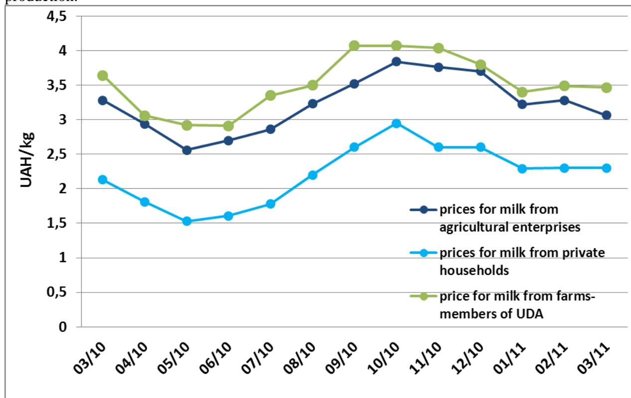
Fig. 1. Dynamics of prices for milk in Ukraine, March 2010 – March 2011 (processing enterprises data)
